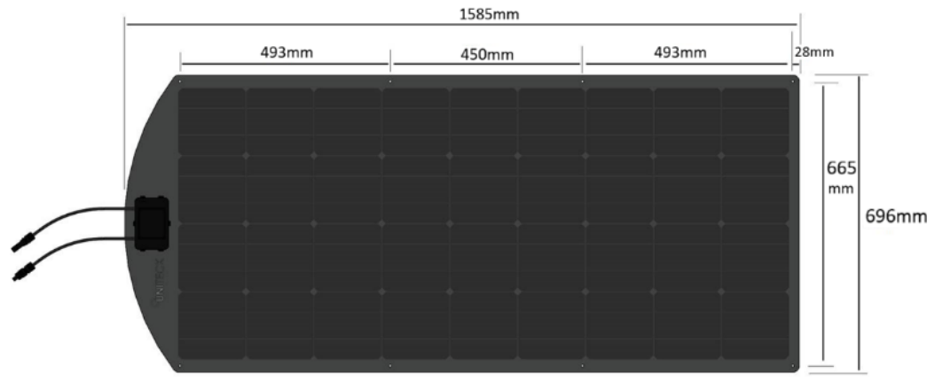
UNISUN 150.12MS
