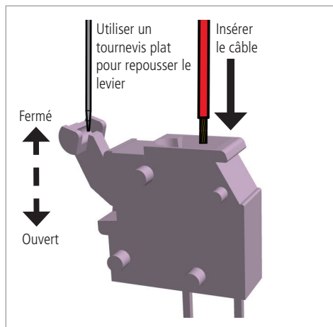
Figure 6: bornes 1 – 17
